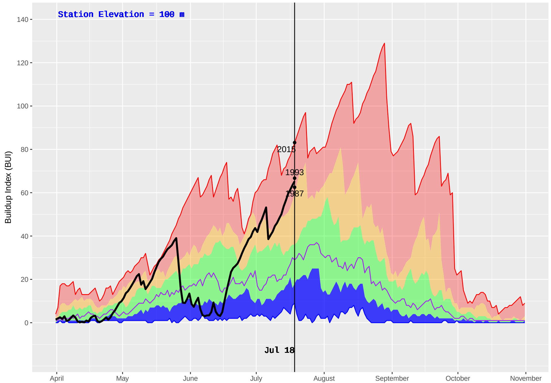
HONNA (93) : Historical (1986–2016) and Current (2018) Daily Buildup Index (BUI)
